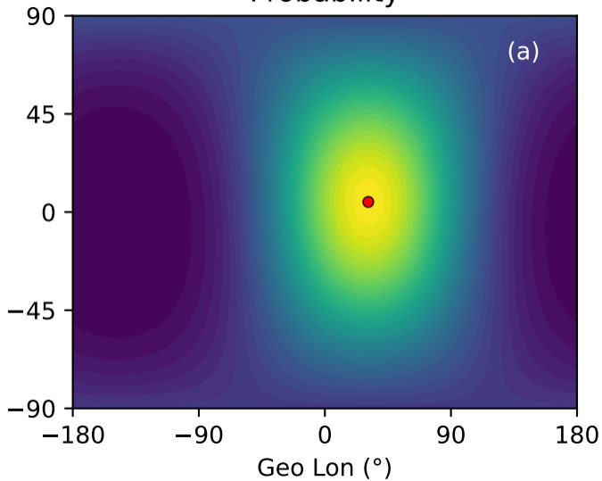
Probability
